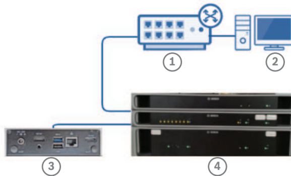
Figure 4.1: Private network connection
